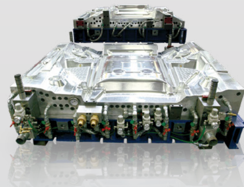
3. CNC-machined aluminium mould and blow-moulded under-bonnet sound absorption shield.
